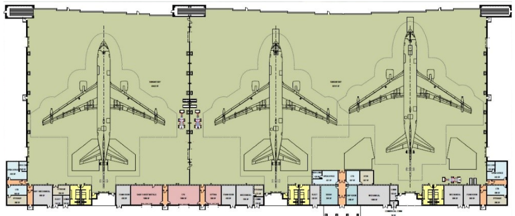
Tinker AFB - KC-46A Three Bay Hangar
